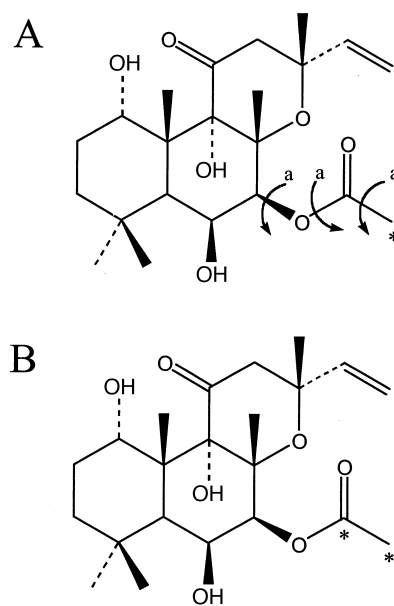
Fig. 1. Structure of forskolin with the sites of isotopic labelling in [7-OCO 13 CH 3 ]-forskolin (A) and [7-O 13 CO 13 CH 3 ]-forskolin (B) indicated with asterisks. Possible bond rotations within the labelled acetyl group are shown (a).
