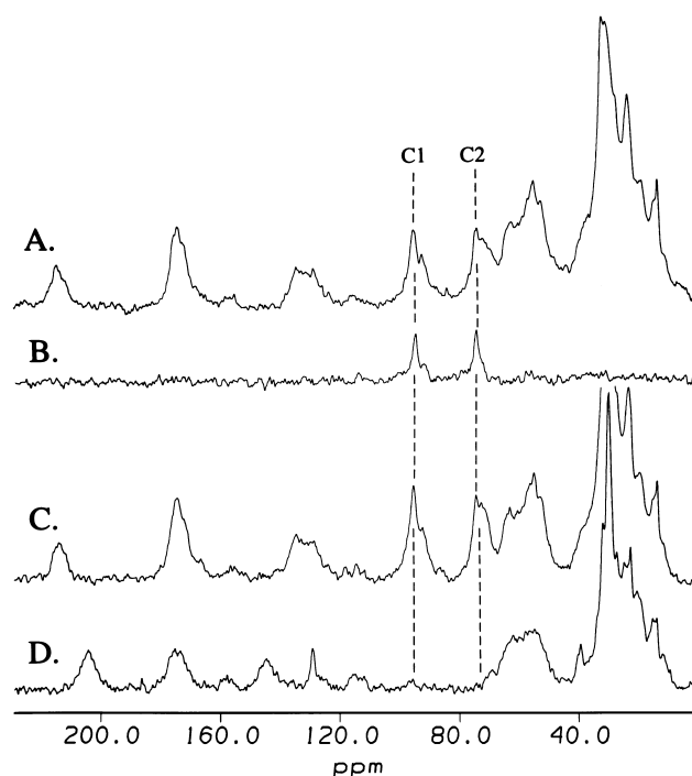
Fig. 5. Measurements recorded at -35^\circ\text{C} for (A) the membranes containing 300 nmol of GalP with 10 mM D-[1,2- ^{13}\text{C}_2 ]glucose by CP MAS, showing strong signal from both positions (C1/C2) labelled within the sugar. (B) Selective detection of substrate in a DQ-filtered spectrum. (C) Substrate detected in a CP MAS spectrum from membranes with 300 nmol of GalP, pretreated with 1 \mu\text{mol} unlabelled forskolin before addition of 10 mM D-[1,2- ^{13}\text{C} ]glucose and (D) the CP MAS spectrum of this sample recorded in a non-frozen state at 2^\circ\text{C} .
